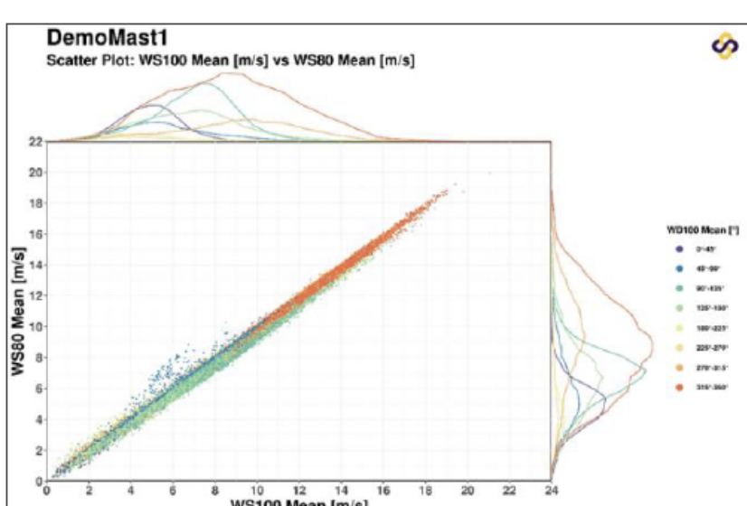
Figure 2-4: Scatter plots of wind speeds at 100m and 80m at Demo Mast 1
