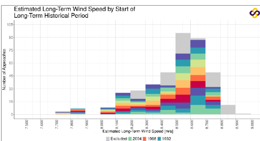
Figure 4-11: Distribution of included and excluded Long-Term Adjustment by historical long-term periods
