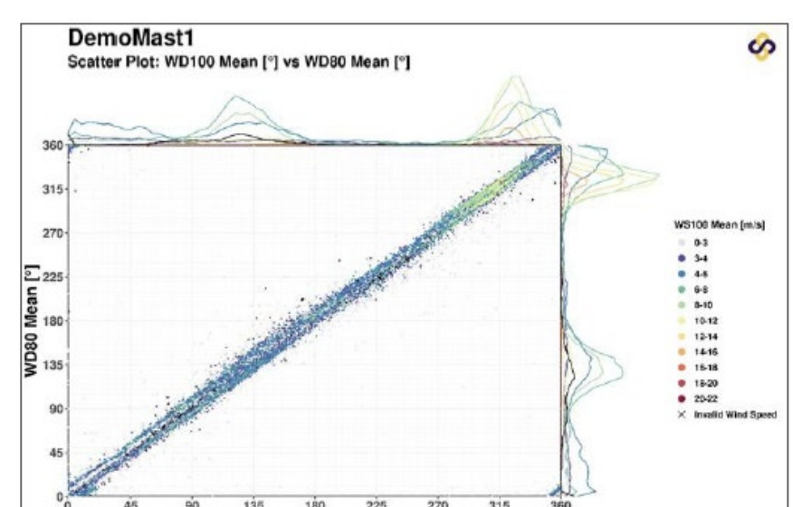
Figure 2-5: Scatter plots of wind direction data at 100m and 80m at Demo Mast 1
