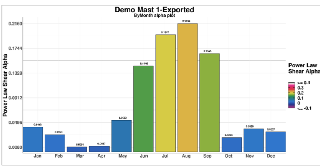
Figure 3-3: Monthly Shear Variation at Demo Mast 1
