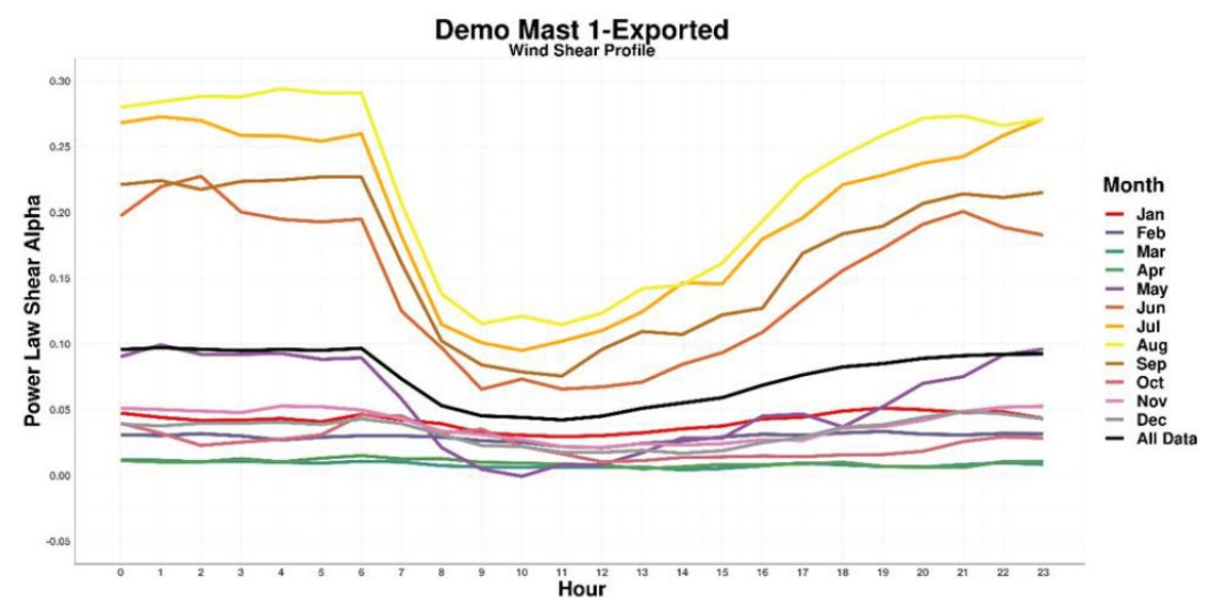
Figure 3-5: Shear Variation by month and hour of the day
